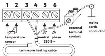
Fig. 2. Mat-mains connection scheme
