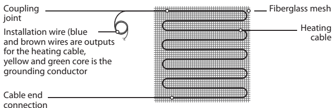
Fig. 1. Mat design
